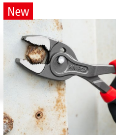
82 01 250 Grips powerfully also large, very tight components with widths across flats of 5 – 27 mm
