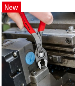
82 01 150 Grips seized components with widths across flats of 3 – 16 mm even in hard-to-reach positions
